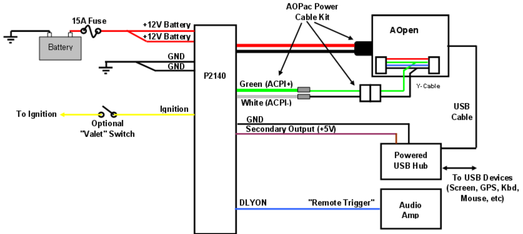
Typical AOpen Pandora Installation (Using AOPac Power Cable Kit)
