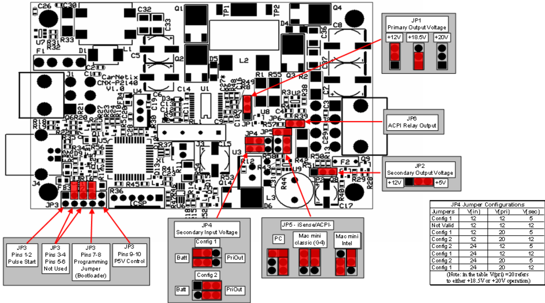
Figure 3 P2140 Jumper Locations and Settings
